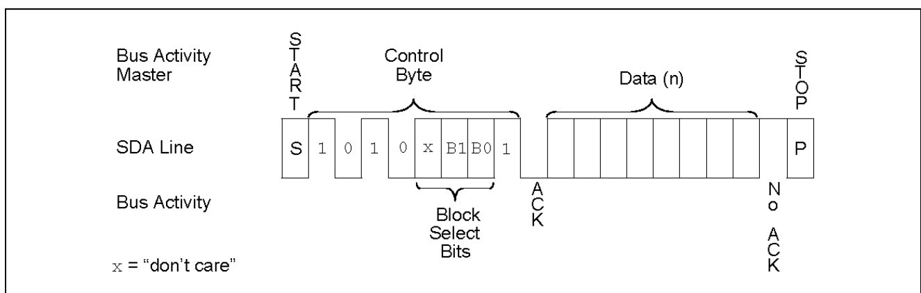
FIGURE 7-1: CURRENT ADDRESS READ
