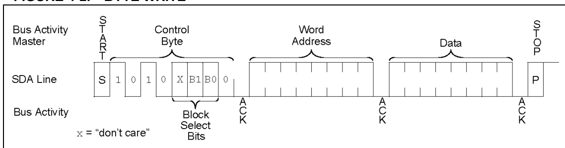
FIGURE 4-1: BYTE WRITE
