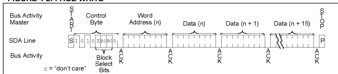
FIGURE 4-2: PAGE WRITE
